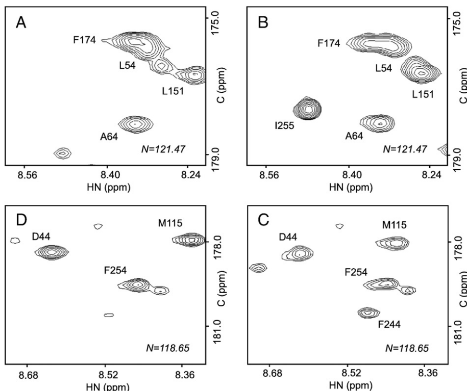
Fig. 6. Line broadening of the backbone amide signals in the HNCO experiment recorded with spin labeled protein (left, A, C) and with the same sample after phenylhydrazine reduction (right, B, D). The upper pair of slices (A, B) is taken at the ^{15}\text{N} shift of 121.5 p.p.m. and the lower pair (C, D) at 118.7 p.p.m. Assigned resonances are labeled.
