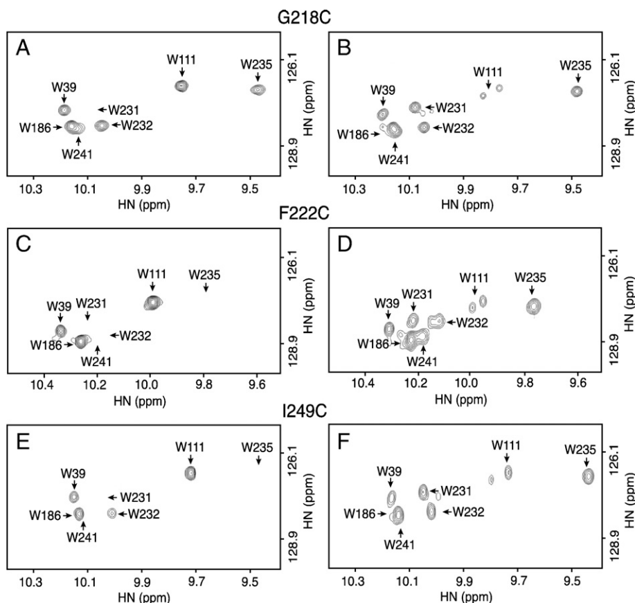
Fig. 5. Line broadening of Trp \epsilon -imino indole signals by PROXYL spin label attached at positions 218 (A, B), 222 (C, D) and 249 (E, F) of subunit a . Spectra of the spin labeled proteins are shown on the left (A, C, E) and the control spectra of the samples reduced with phenylhydrazine on the right (B, D, F). Resonance assignments are indicated by the arrows.
