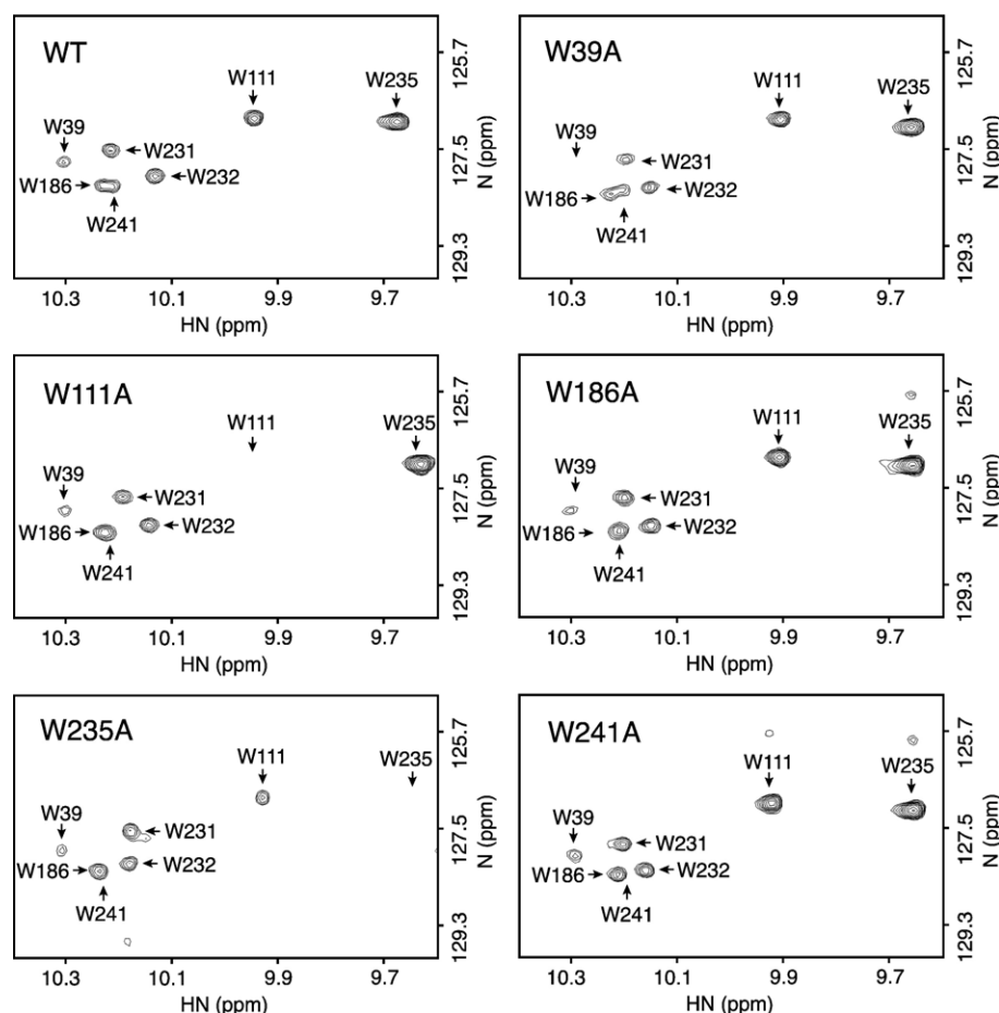
Fig. 2. Examples of the assignment of the \epsilon -imino indole signal of Trp residues by comparing the spectra of wild type and single W \rightarrow A substituted mutants. The positions of Trp signals in the spectrum of wild type protein are indicated by the labeled arrows.
