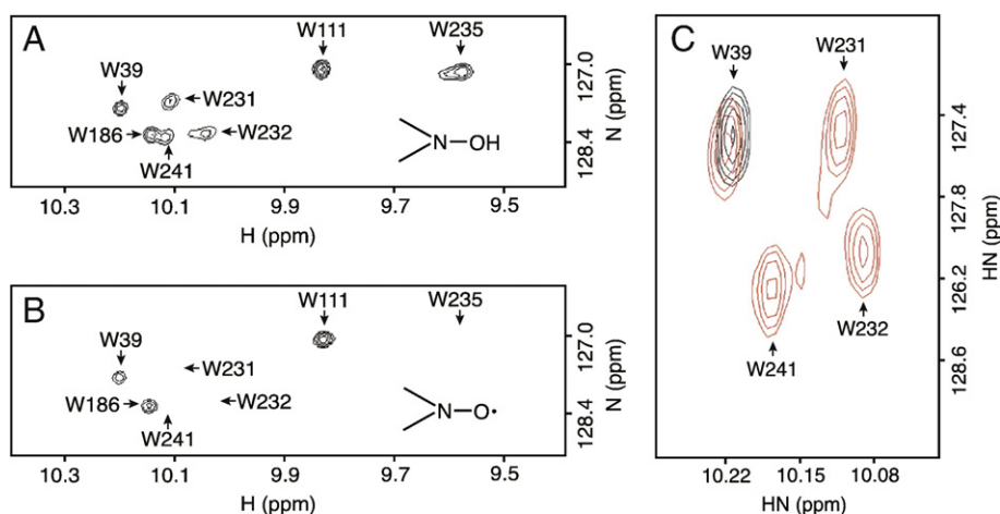
Fig. 3. Line broadening of Trp \epsilon -imino indole signals by PROXYL spin label attached at Cys223 of the subunit a . (A) Control spectrum of wild type protein recorded after reducing the PROXYL spin label with phenylhydrazine. Resonance assignments are indicated by the arrows. (B) PROXYL labeled wild type sample showing loss of W231, W232, W235 and W241 resonances. (C) Overlay of the spectra of the spin labeled W186F variant of subunit a (black) and of the phenylhydrazine reduced sample [red].
